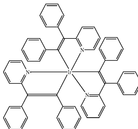
COMPOUND 2
