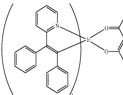
COMPOUND 2
